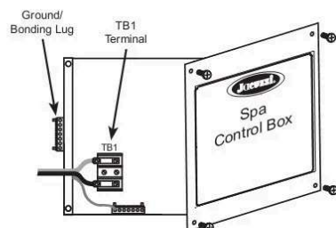
Figure 11 The Control Box for 3-wire, 240 VAC connection
