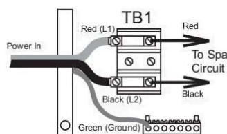
Figure 12 3-Wire, 240 VAC Connection for Models J-235, J-245, J-275, J-280, J-335, J-345, J-355, J-365, J-375, (For hard-wired connections only)
