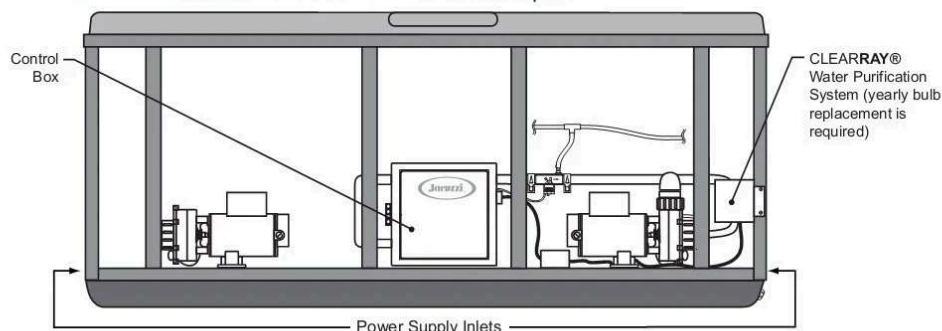
Figure 10 Spa Equipment Compartment (spa features subject to change without notice)
